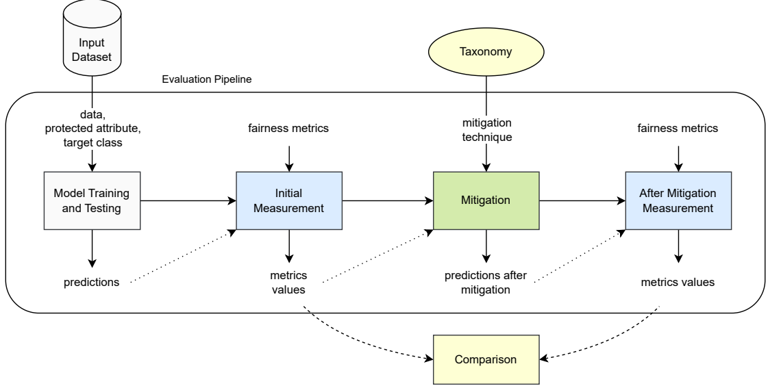
Figure 1: Proposed evaluation pipeline for testing and comparing fairness mitigation techniques.
